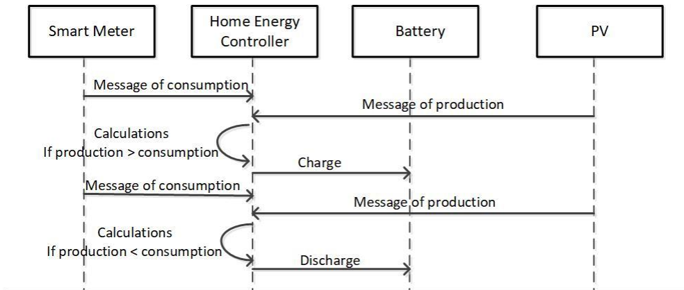
Figure 31. Message Sequence Chart for UC 2 - Self-consumption of on-site produced RES energy.
