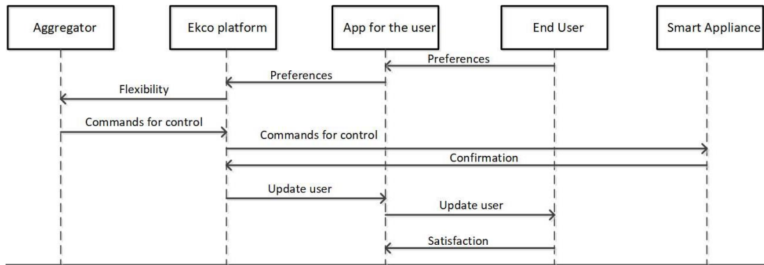
Figure 50. Message Sequence Chart for UC 2 – Information control (control by aggregator).
