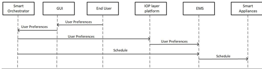
Figure 38. Message Sequence Chart for PUC 2.
