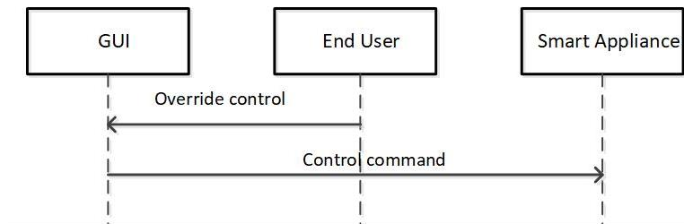
Figure 42. Message Sequence Chart for PUC 6.
