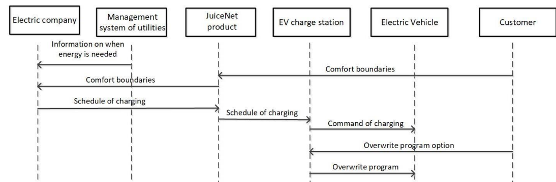
Figure 22. Message Sequence Chart for UC 5 – United States (California).
