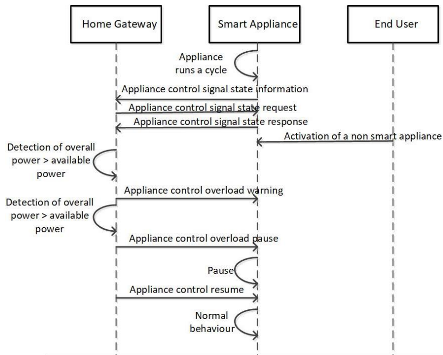
Figure 53. Message Sequence Chart for UC 3 – Control of smart appliance in case of overload.
