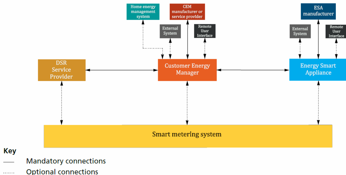
Figure 11. Representation of system level CEM-ESA energy flexibility architecture with separate CEM/ESAG.
