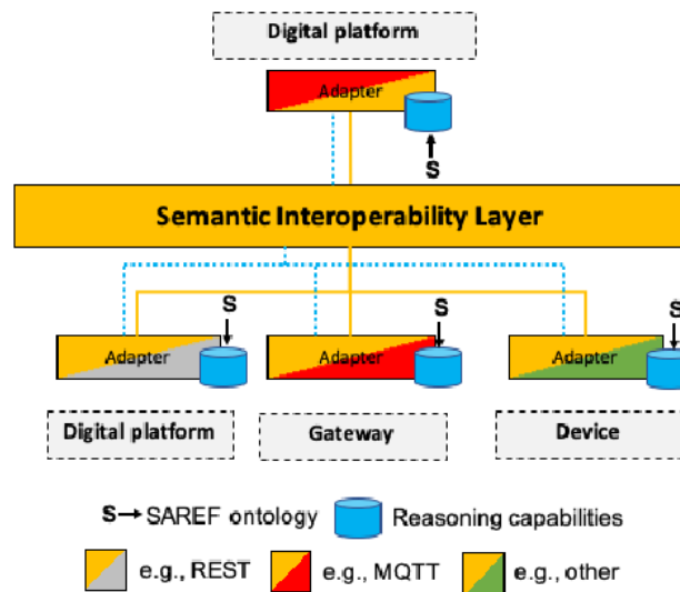
Figure 10. Interconnect Adapter: High level overview of the concept.
