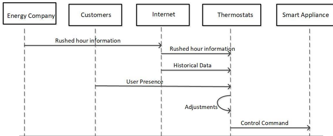
Figure 21. Message Sequence Chart for UC 4 – United States (Austin).
