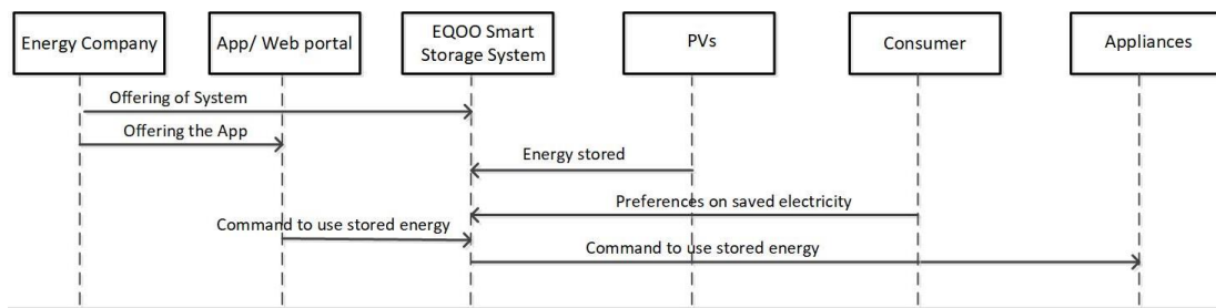
Figure 26. Message Sequence Chart for UC 1 – Germany (Cuxhaven Region – Lower Saxony).
