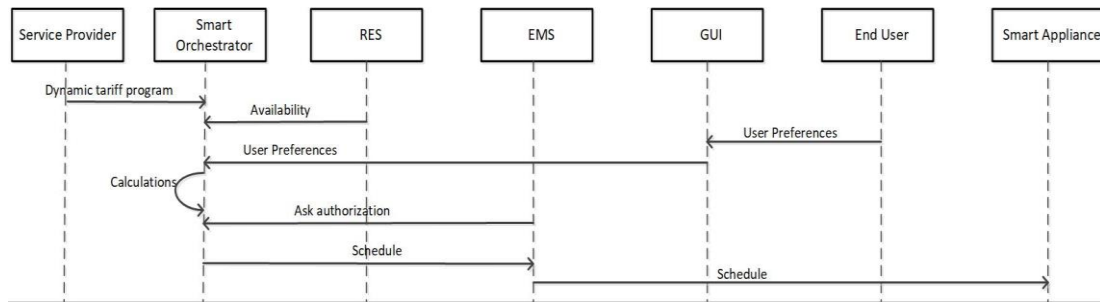
Figure 41. Message Sequence Chart for PUC 5.
