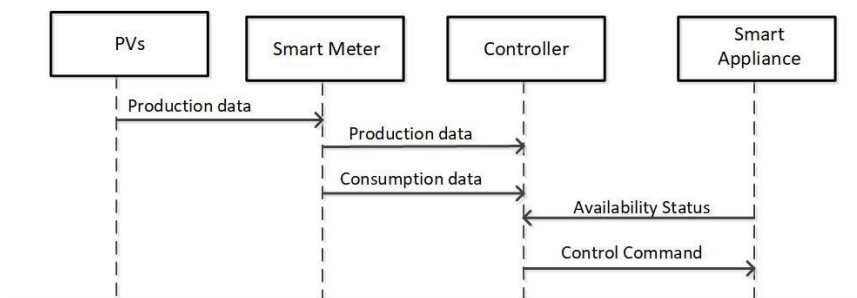
Figure 58. Message Sequence Chart for the generic use case of local optimal energy consumption.
