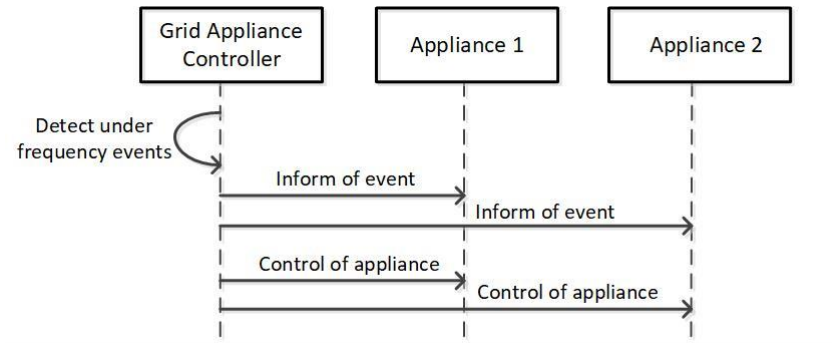
Figure 29. Message Sequence Chart for UC 2 – United States (Pacific Northwest).
