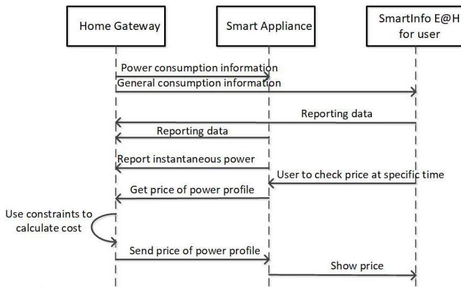
Figure 51. Message Sequence Chart for UC 1 – Visualization of consumption data.
