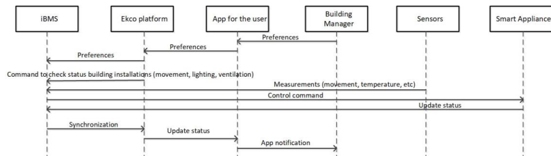
Figure 49. Message Sequence Chart for UC 2 – Information control (control by building manager).
