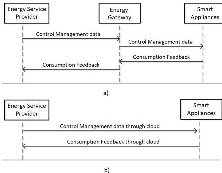
Figure 13. Message sequence chart for generic Use Case, a) Communication of energy smart appliances through the home energy gateway, b) Communication of energy smart appliances directly to the energy service provider through the cloud.
