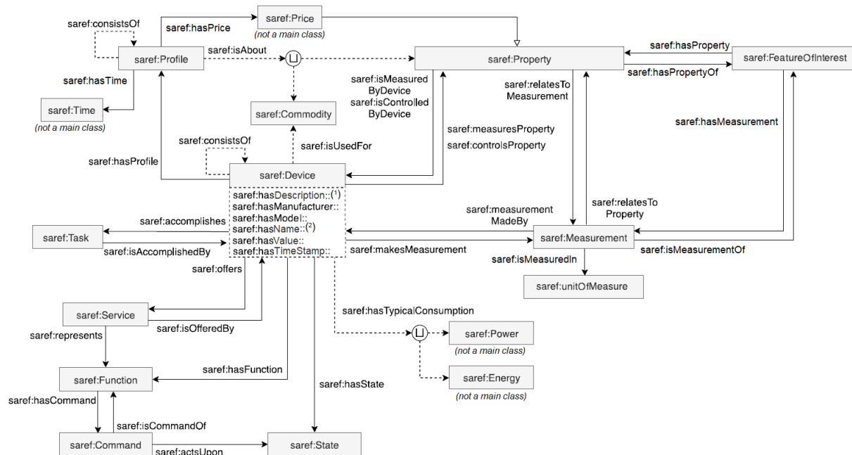
Figure 55. Overview of the main classes of the SAREF ontology.
