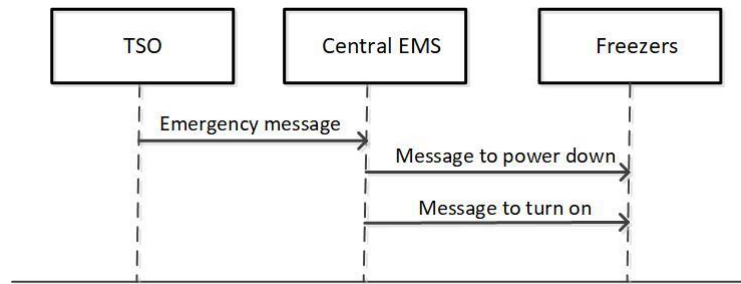
Figure 35. Message Sequence Chart for UC 6 - Frequency restoration reserves based on commercial refrigeration.
