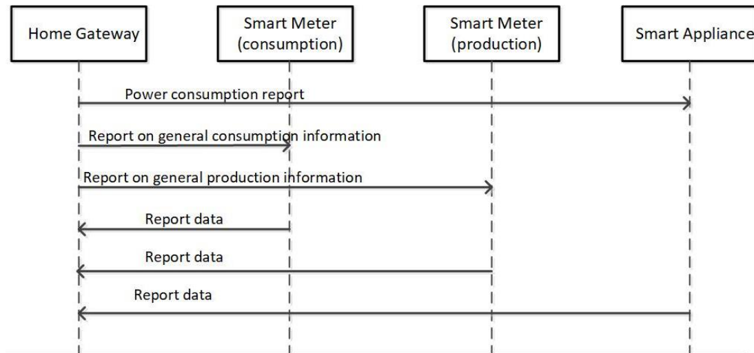
Figure 54. Message Sequence Chart for UC 4 – Interaction of smart meter.
