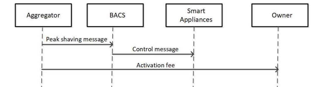
Figure 36. Message Sequence Chart for UC 7 - Peak shaving combined with energy efficiency by appliances controlled by a building automation and control system.
