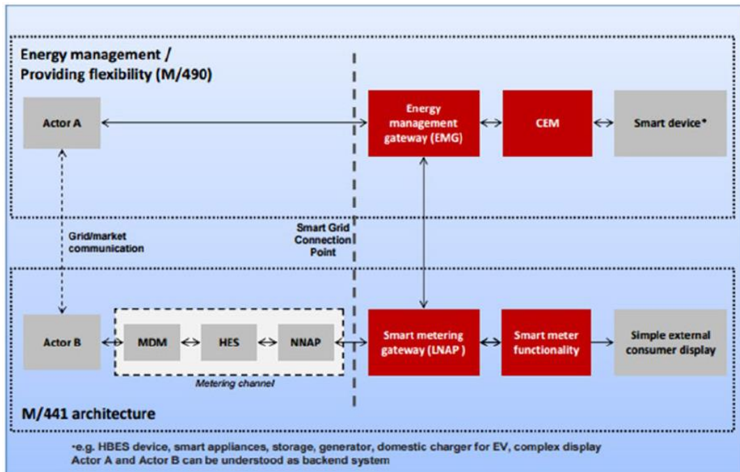
Figure 2. Flexibility functional architecture as proposed by the CEN-CENELEC-ETSI Smart Grid Coordination Group.
