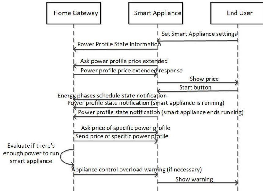
Figure 52. Message Sequence Chart for UC 2 – Setting of a smart appliance according to price tariffs.
