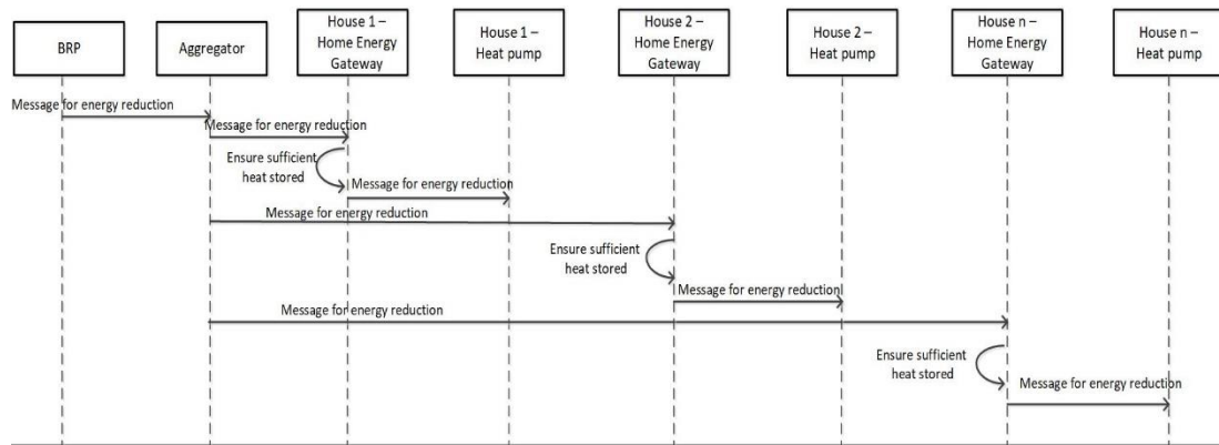
Figure 30. Message Sequence Chart for UC 1 – Load shifting of heat pump supplied houses.
