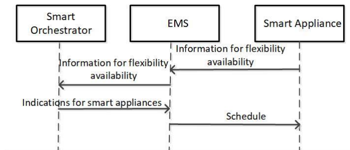
Figure 40. Message Sequence Chart for PUC 4.
