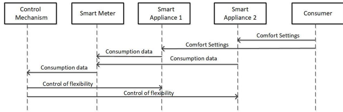
Figure 28. Message Sequence Chart for UC 1 – Belgium (Flemish region).
