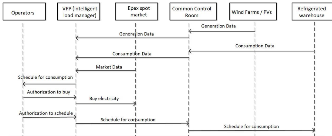
Figure 20. Message Sequence Chart for UC 3 – Germany.
